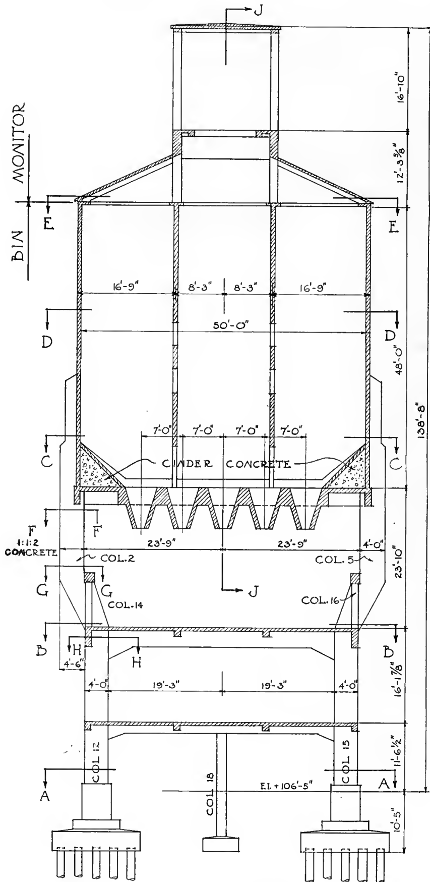
CROSS SECTION SHOWING CENTER WALL BETWEEN BINS
